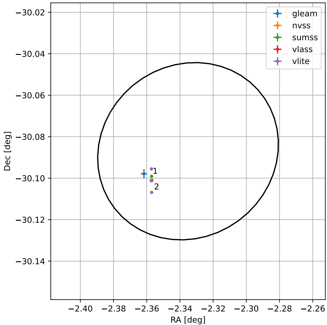
4FGL J2350.6-3005
