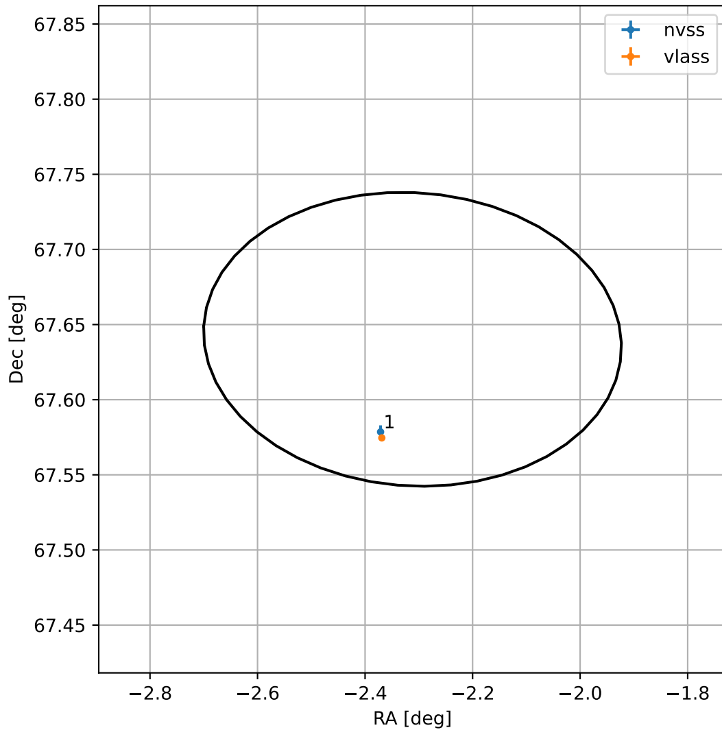
4FGL J2350.7+6738
