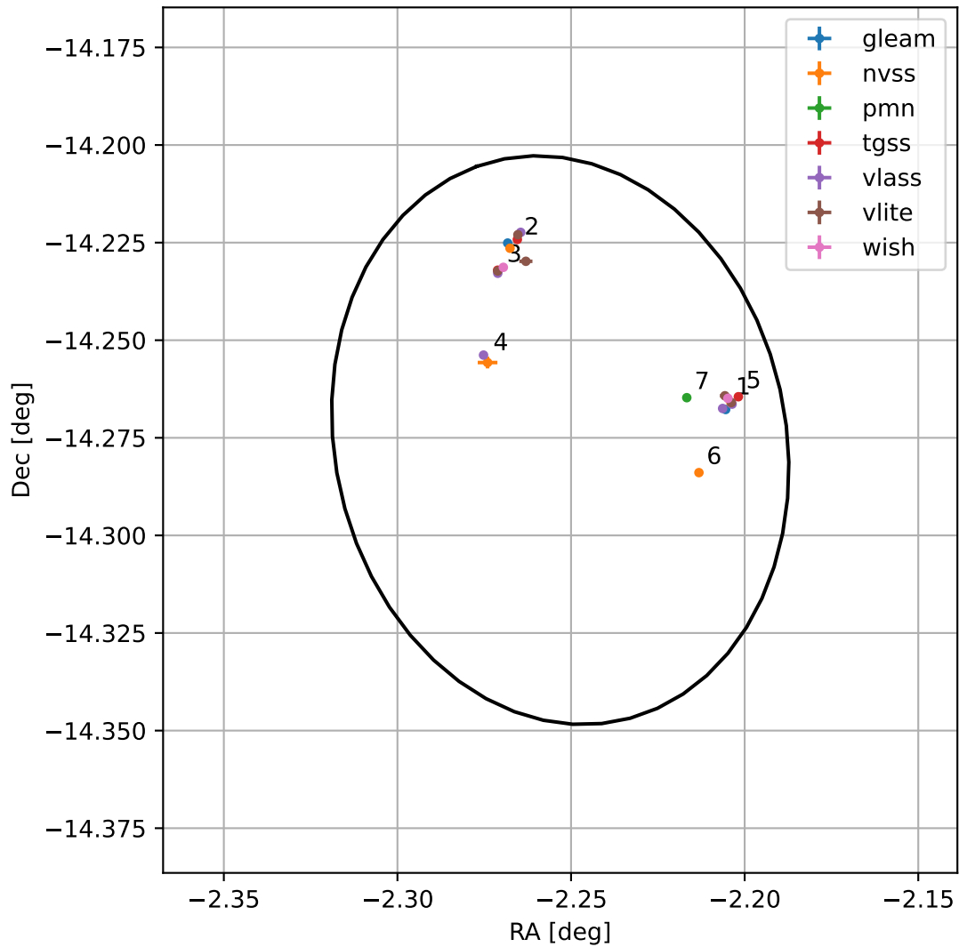
4FGL J2350.9-1416
