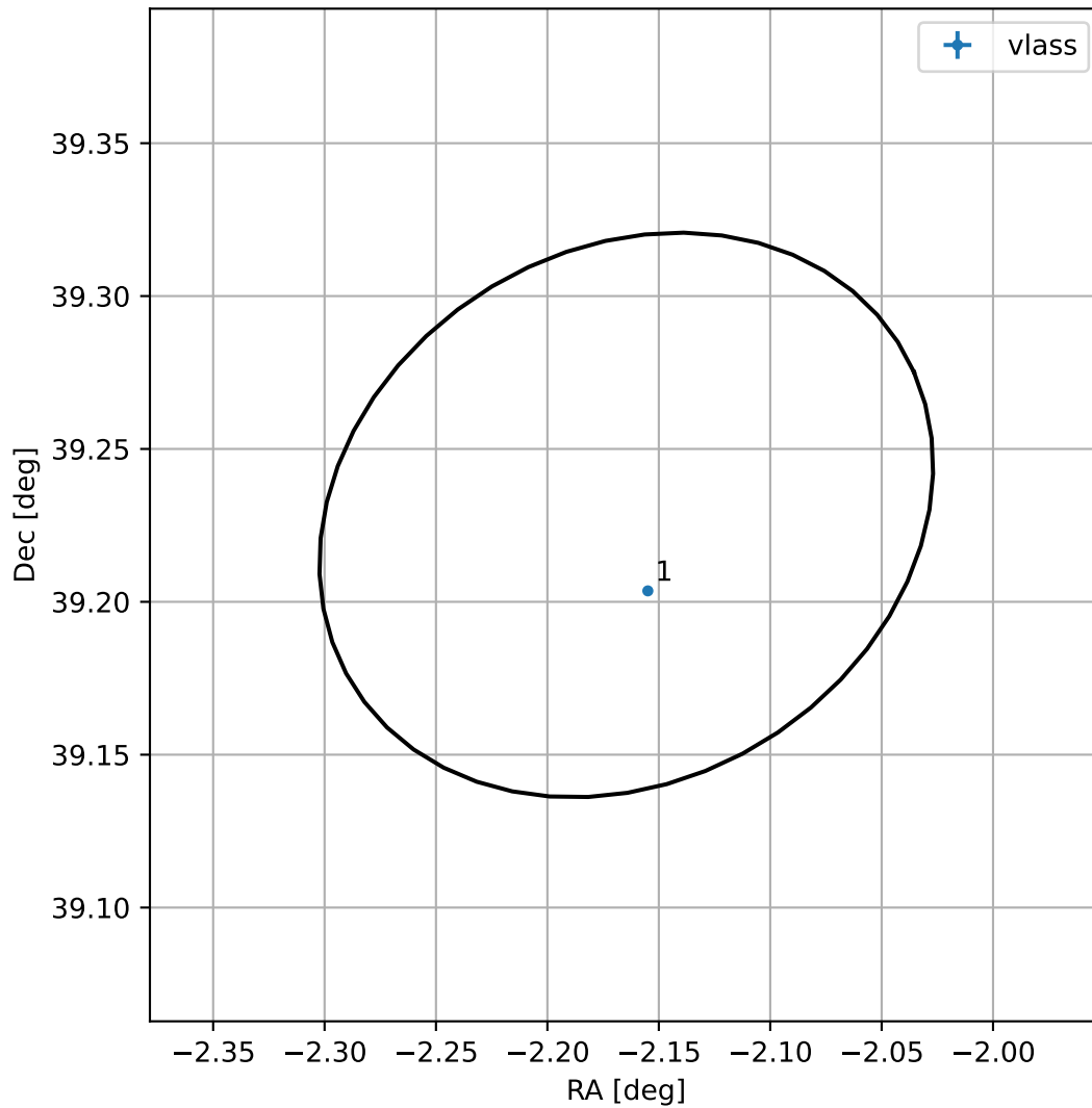
4FGL J2351.3+3913
