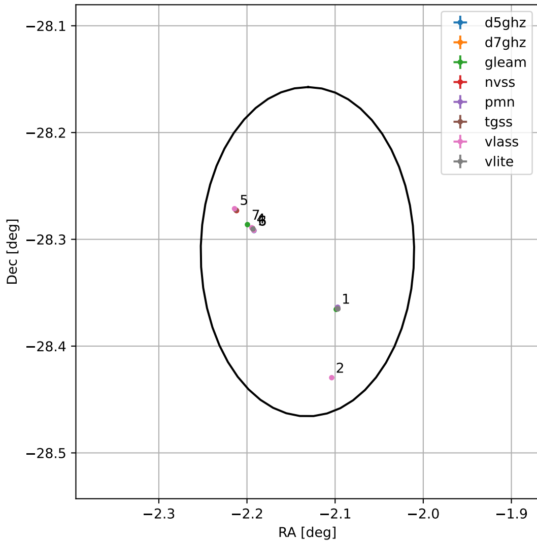
4FGL J2351.4-2818
