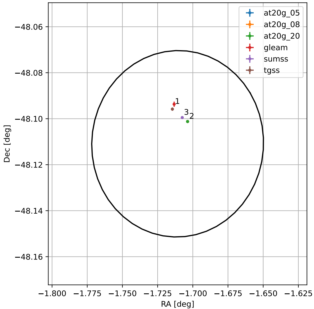
4FGL J2353.1-4806
