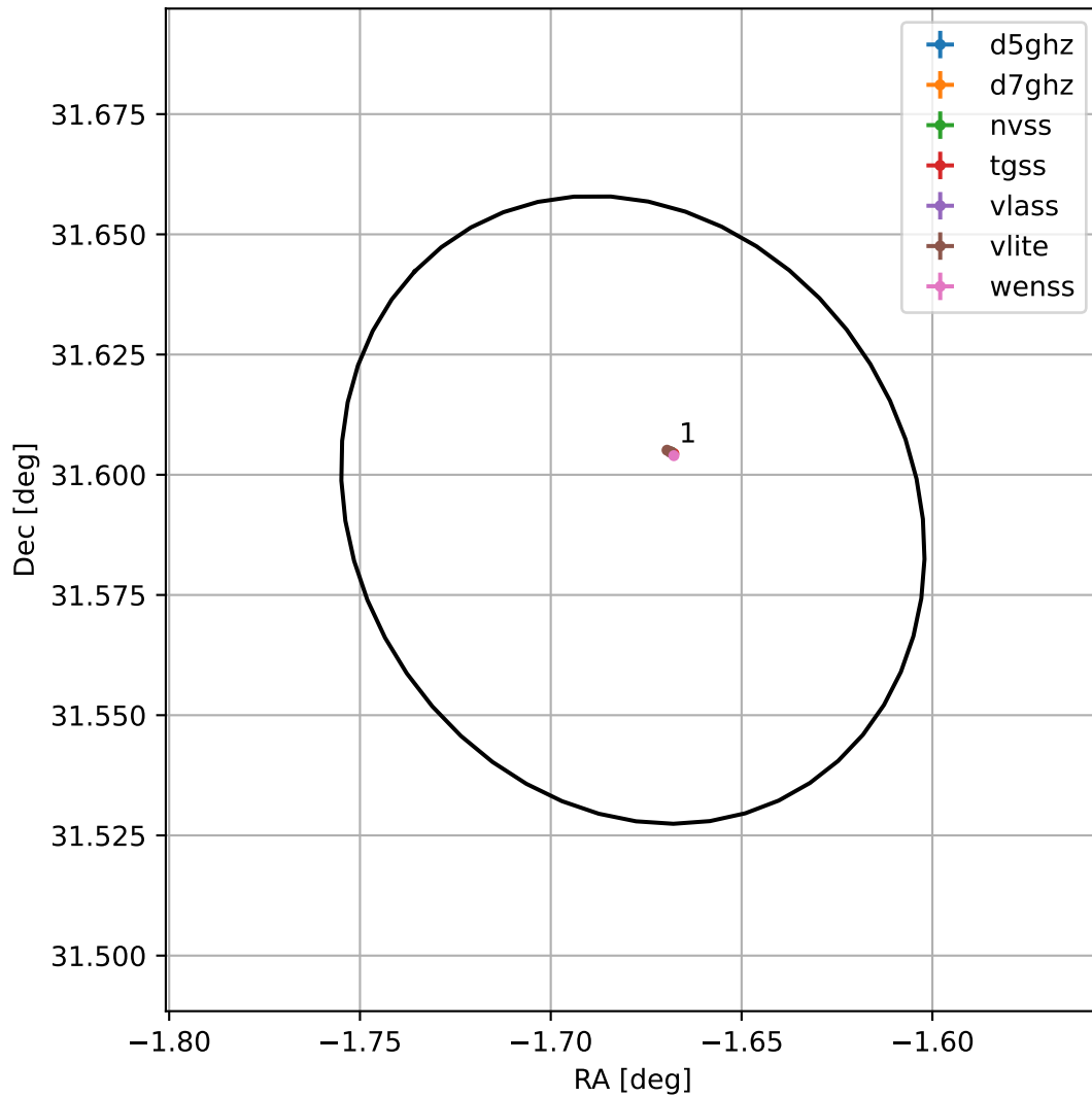
4FGL J2353.2+3135
