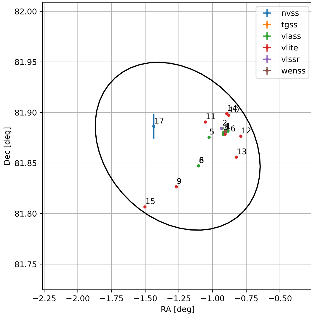
4FGL J2354.9+8151
