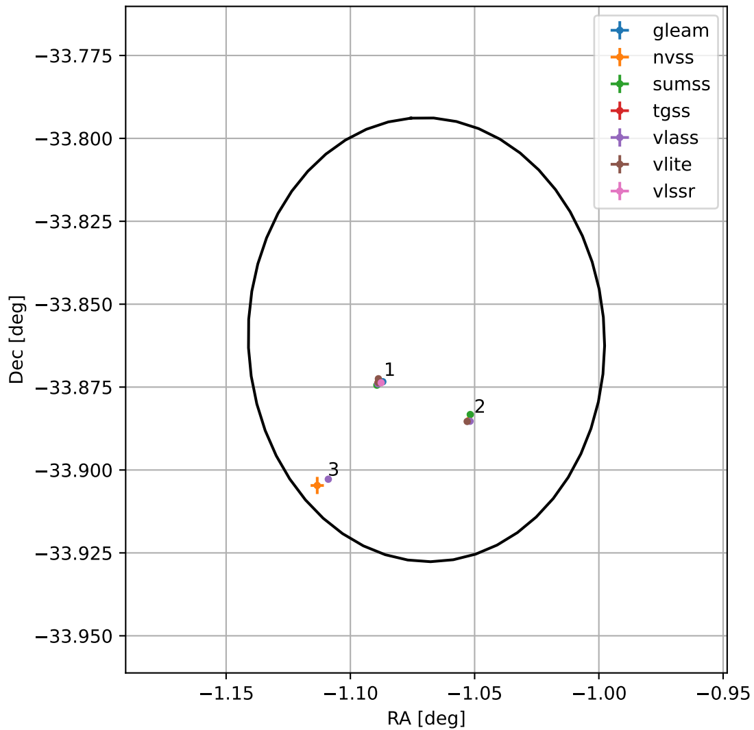
4FGL J2355.7-3351
