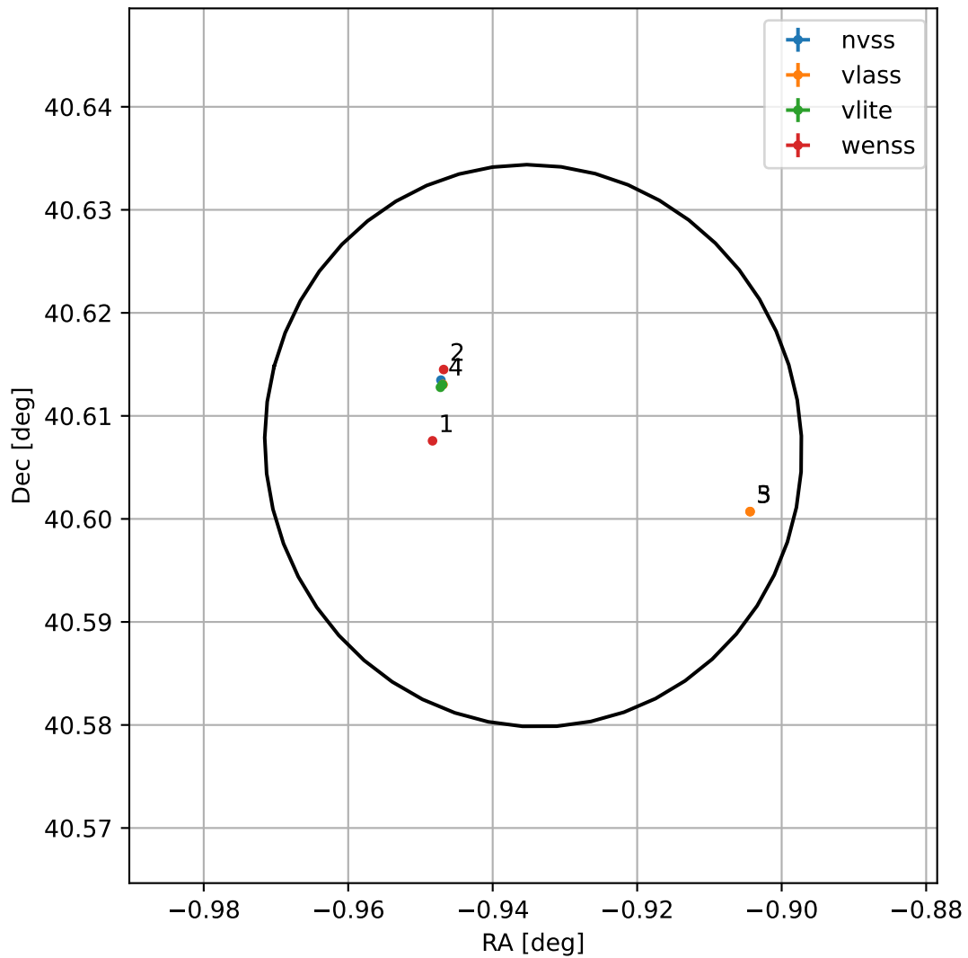
4FGL J2356.2+4036
