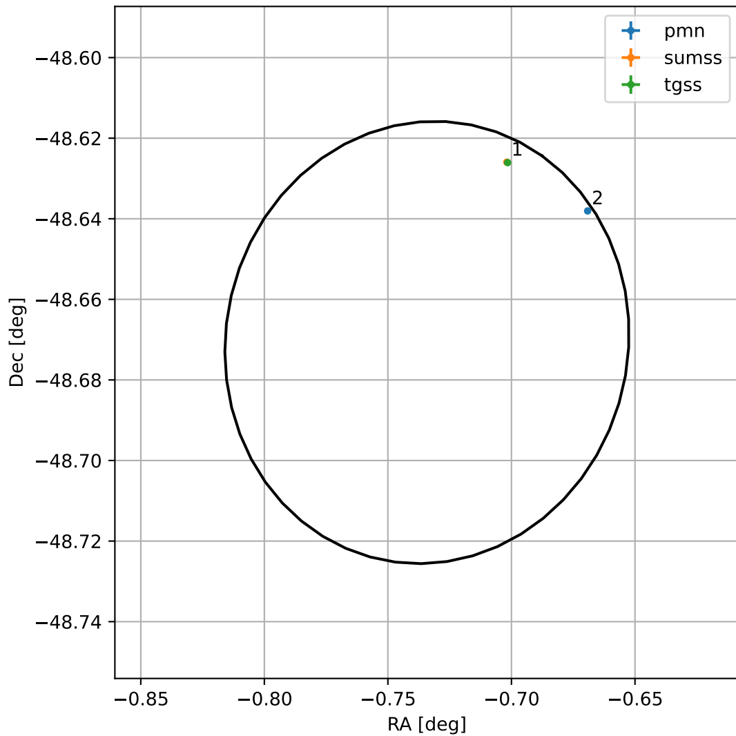
4FGL J2357.0-4840
