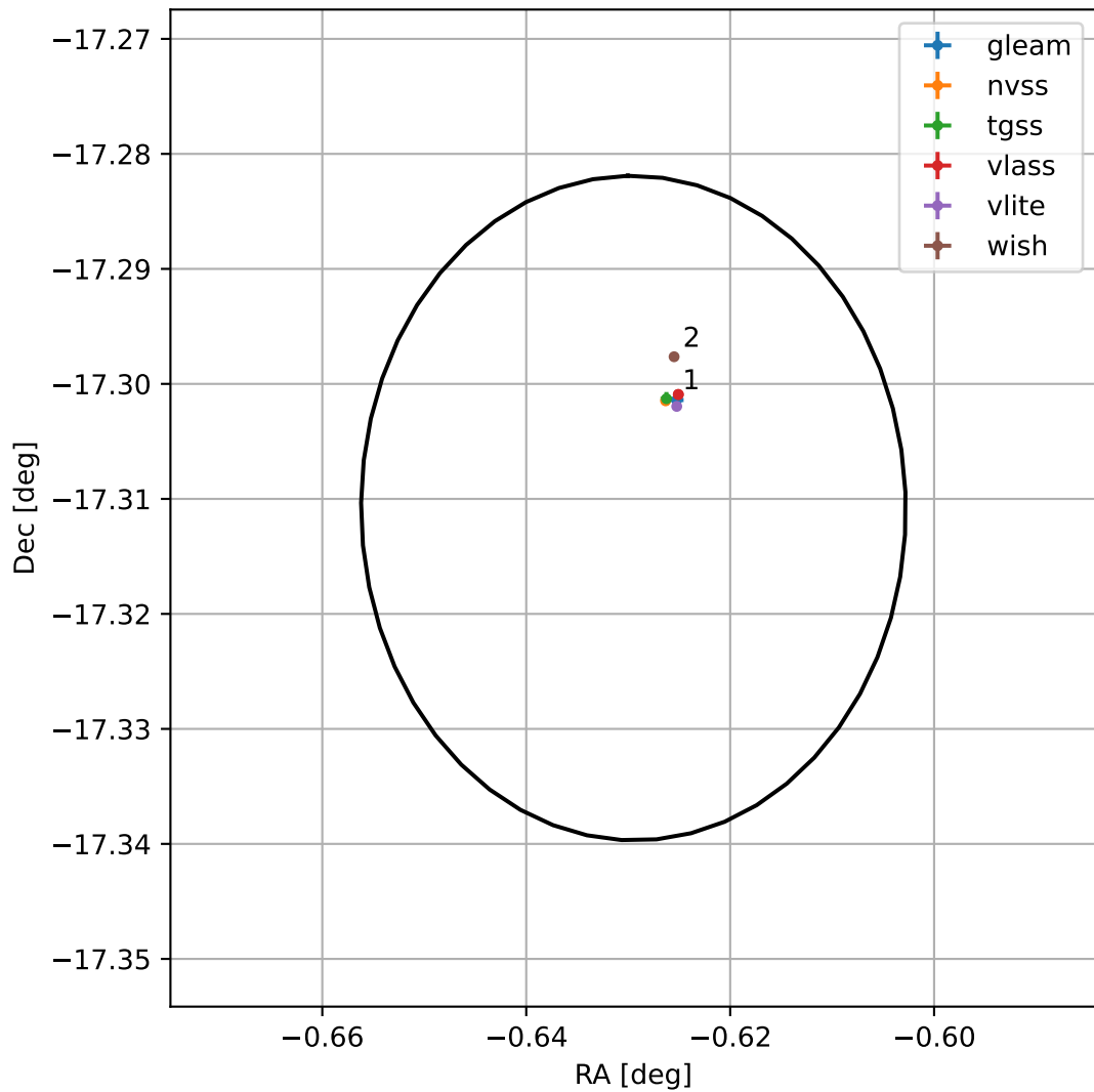
4FGL J2357.4-1718
