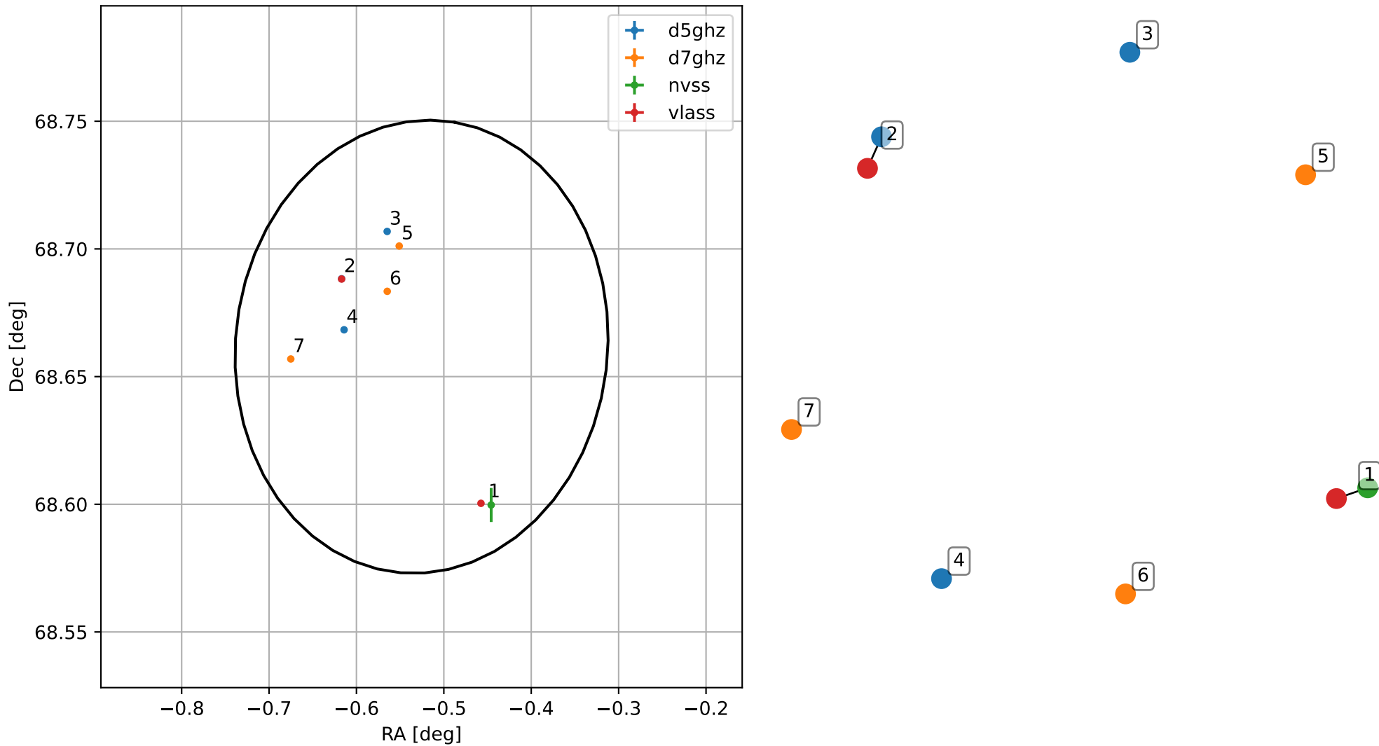
4FGL J2357.8+6839
