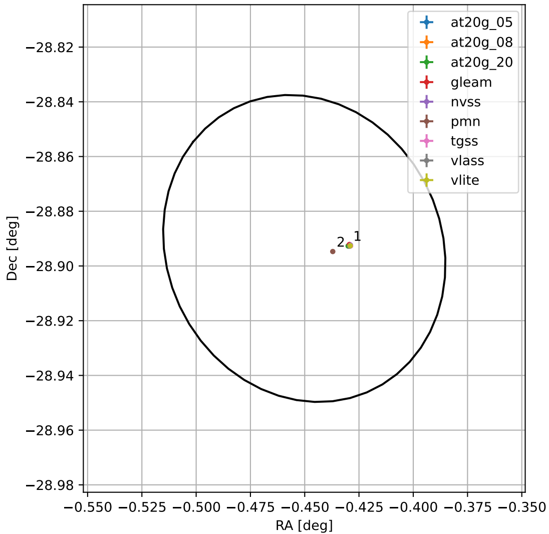
4FGL J2358.1-2853
