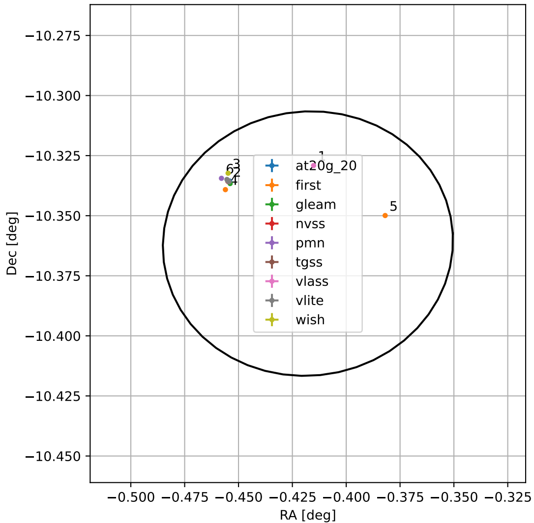
4FGL J2358.3-1021
