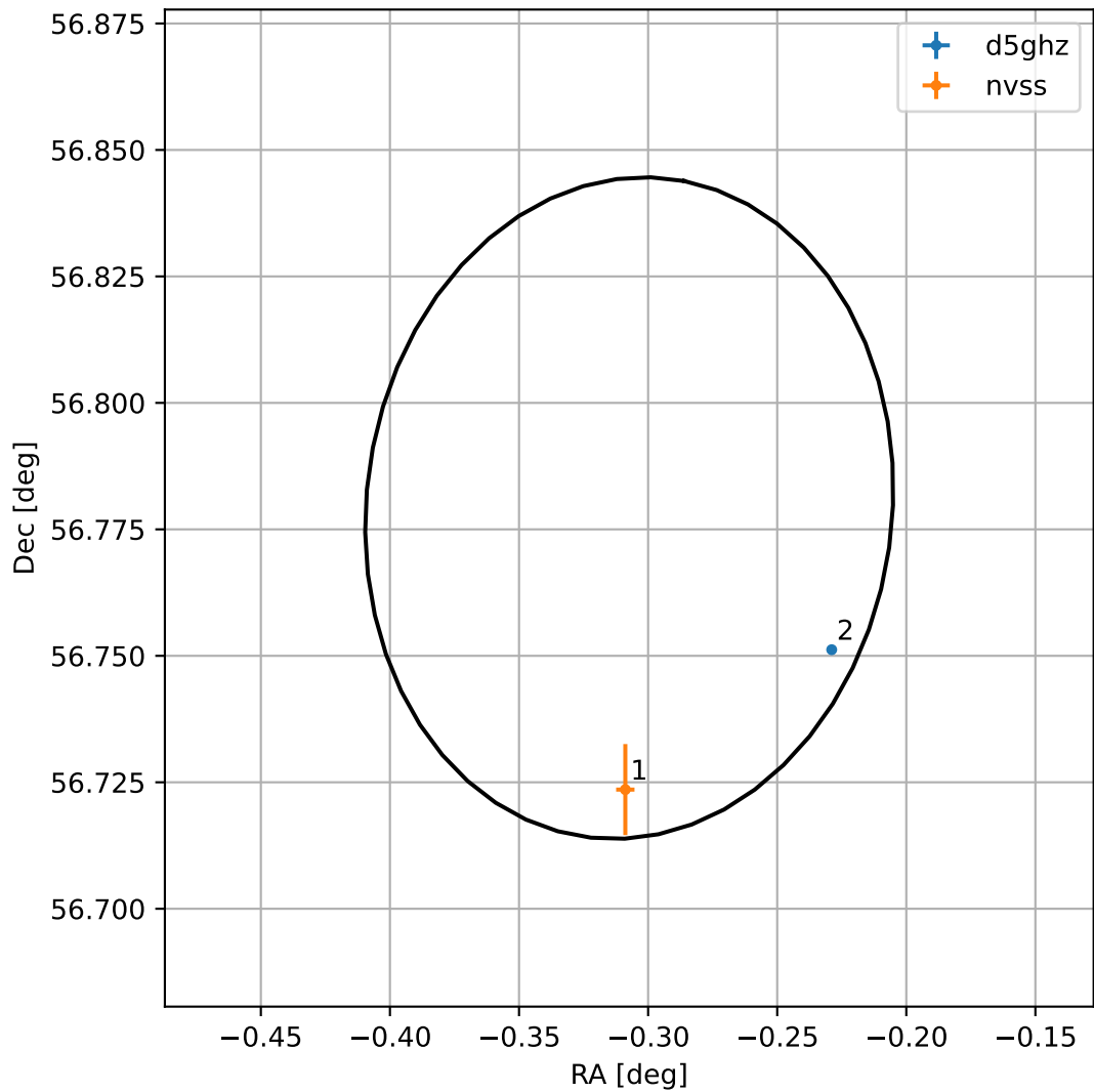
4FGL J2358.7+5646
