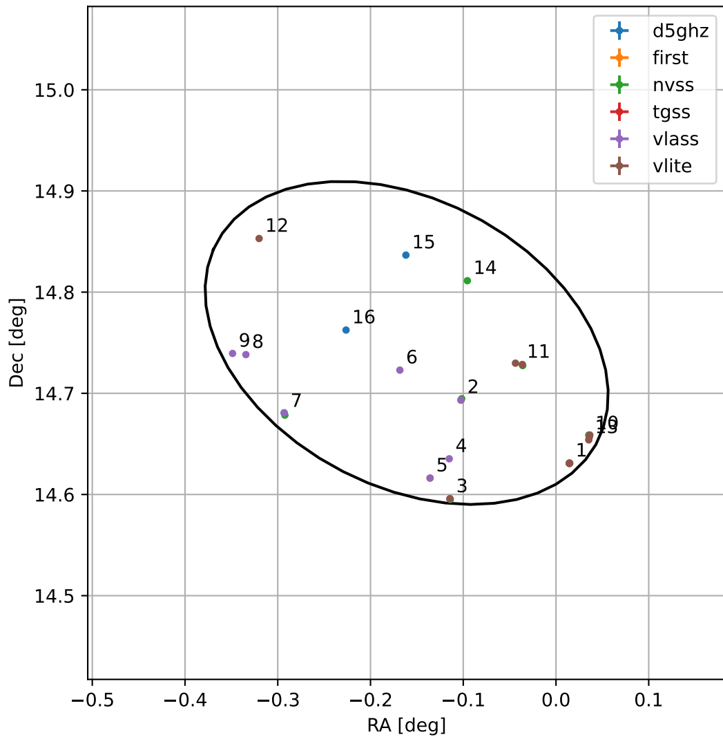
4FGL J2359.3+1444
