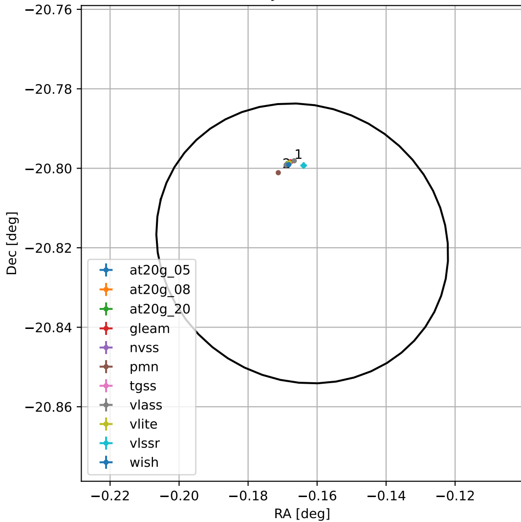
4FGL J2359.3-2049
