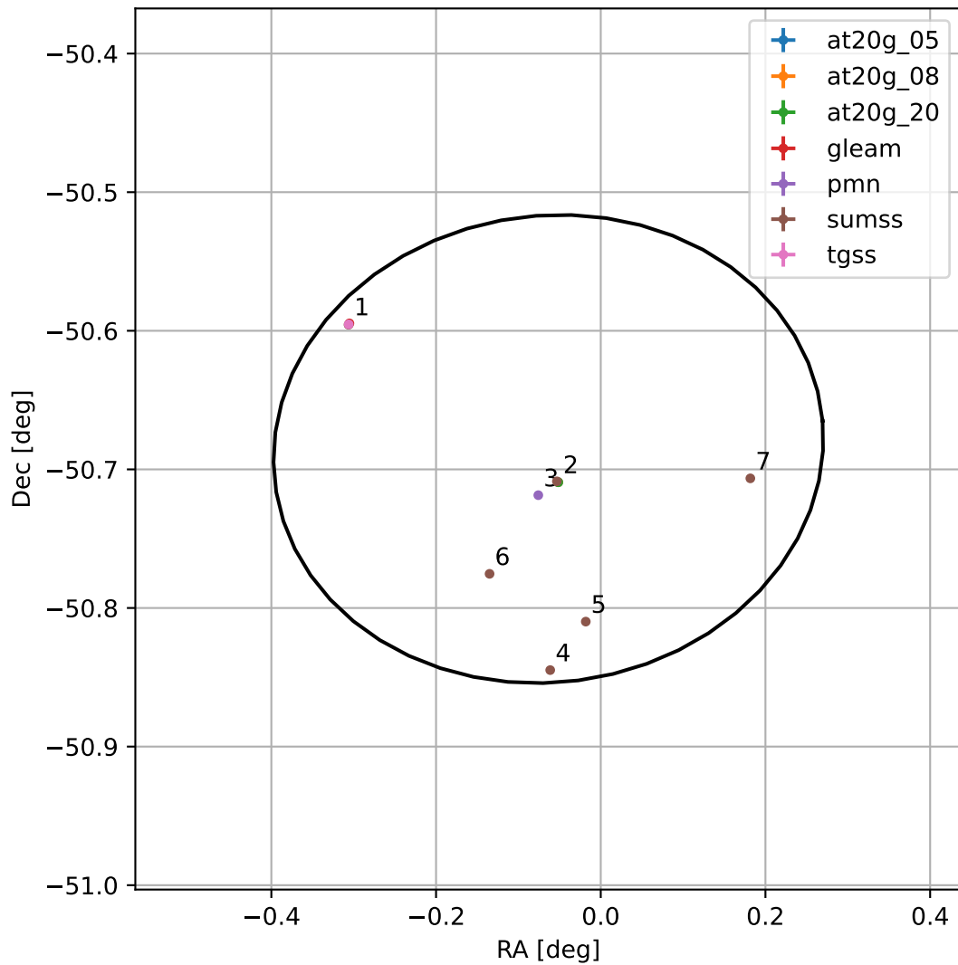
4FGL J2359.7-5041
