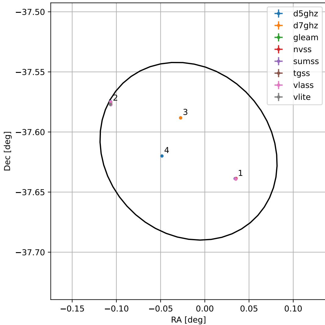
4FGL J2359.9-3736
