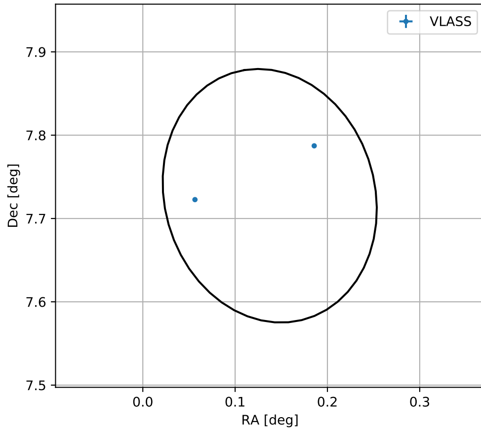
4FGL J0000.5+0743
