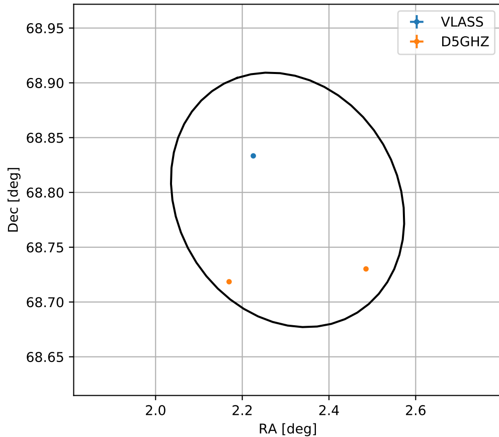
4FGL J0009.2+6847
