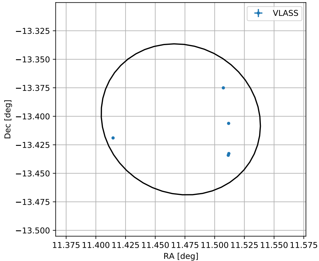
4FGL J0045.8-1324
