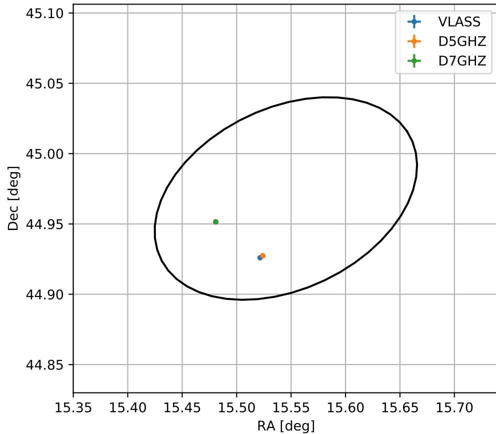
4FGL J0102.1+4458
