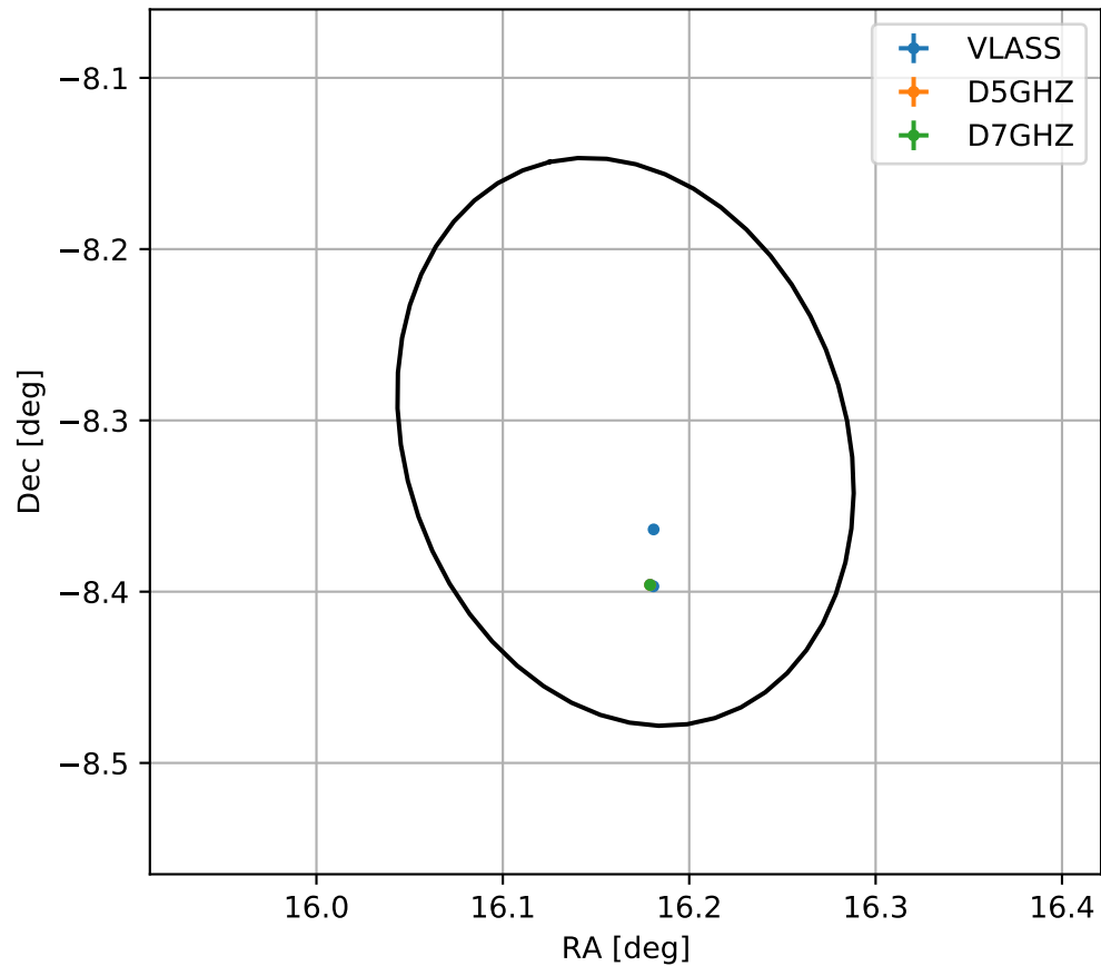
4FGL J0104.6-0818
