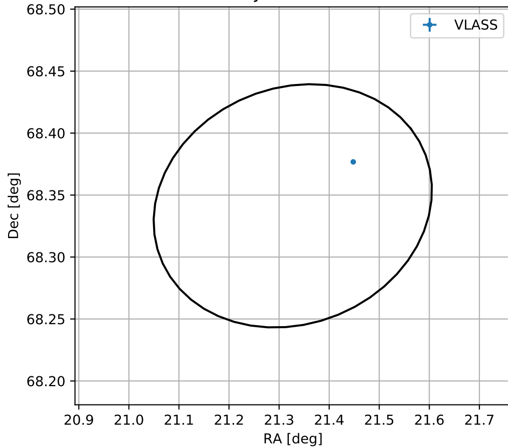
4FGL J0125.3+6820
