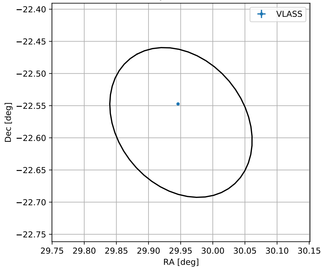
4FGL J0159.8-2234
