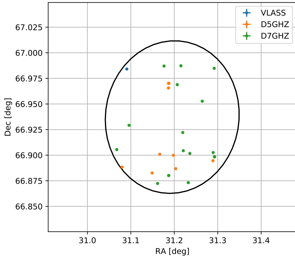
4FGL J0204.7+6656
