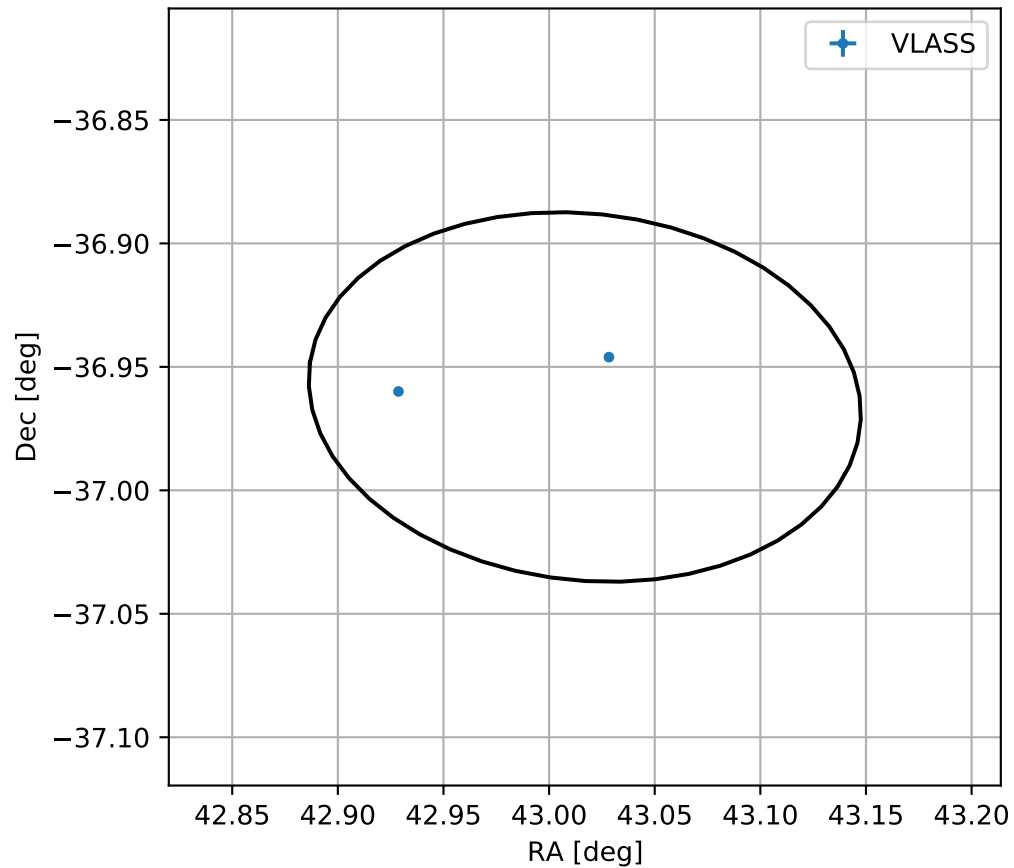
4FGL J0252.0-3657
