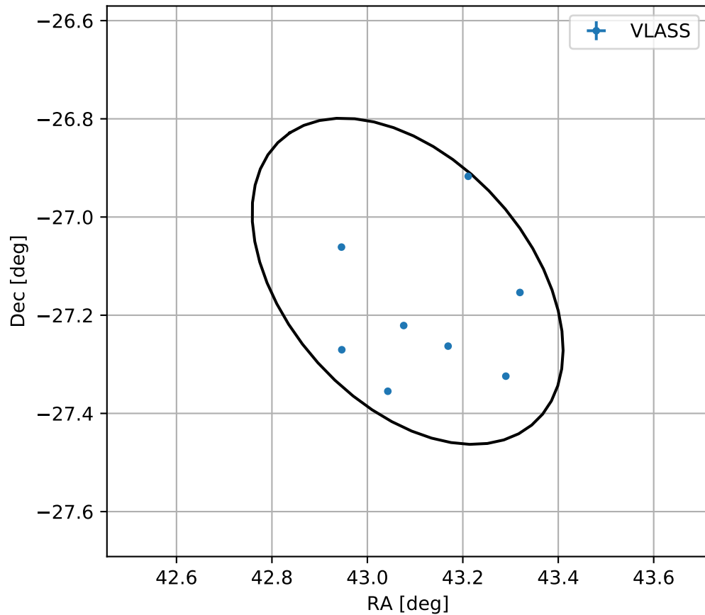
4FGL J0252.3-2707
