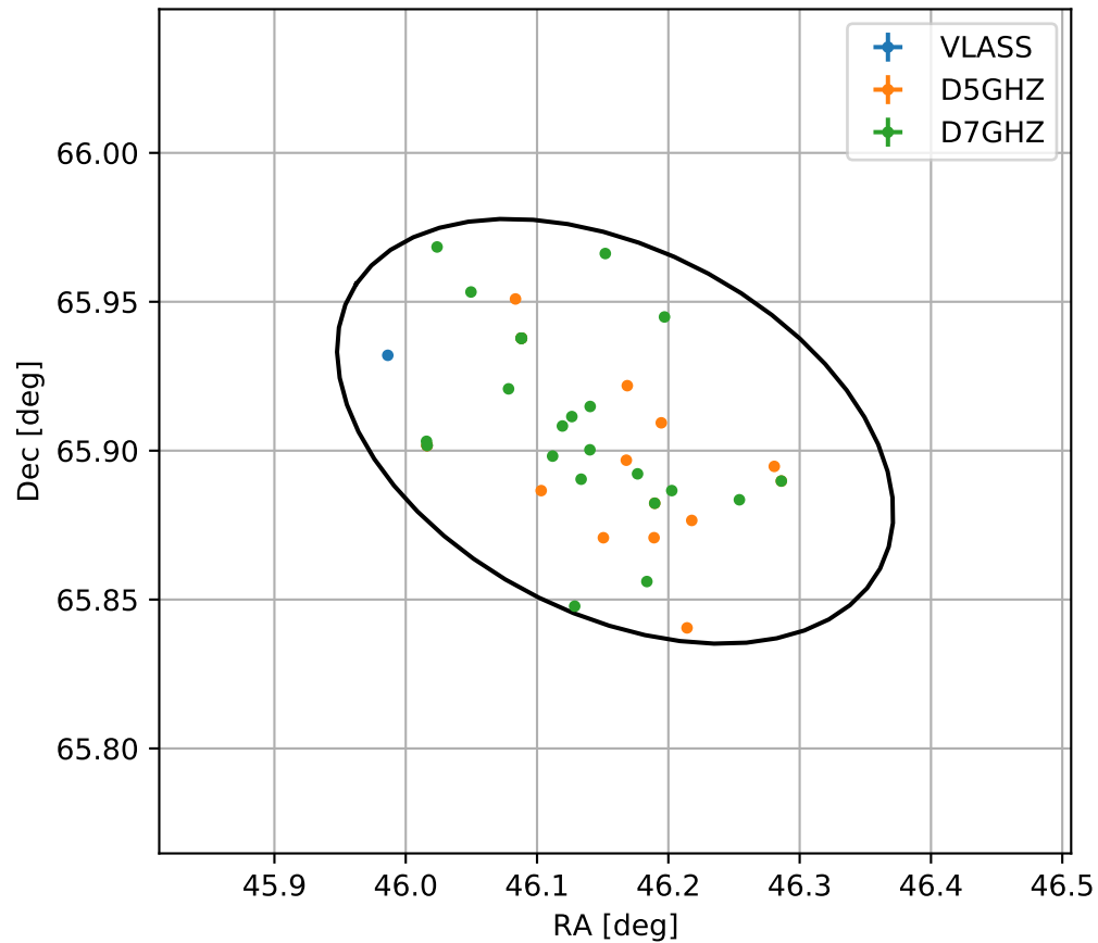
4FGL J0304.6+6554
