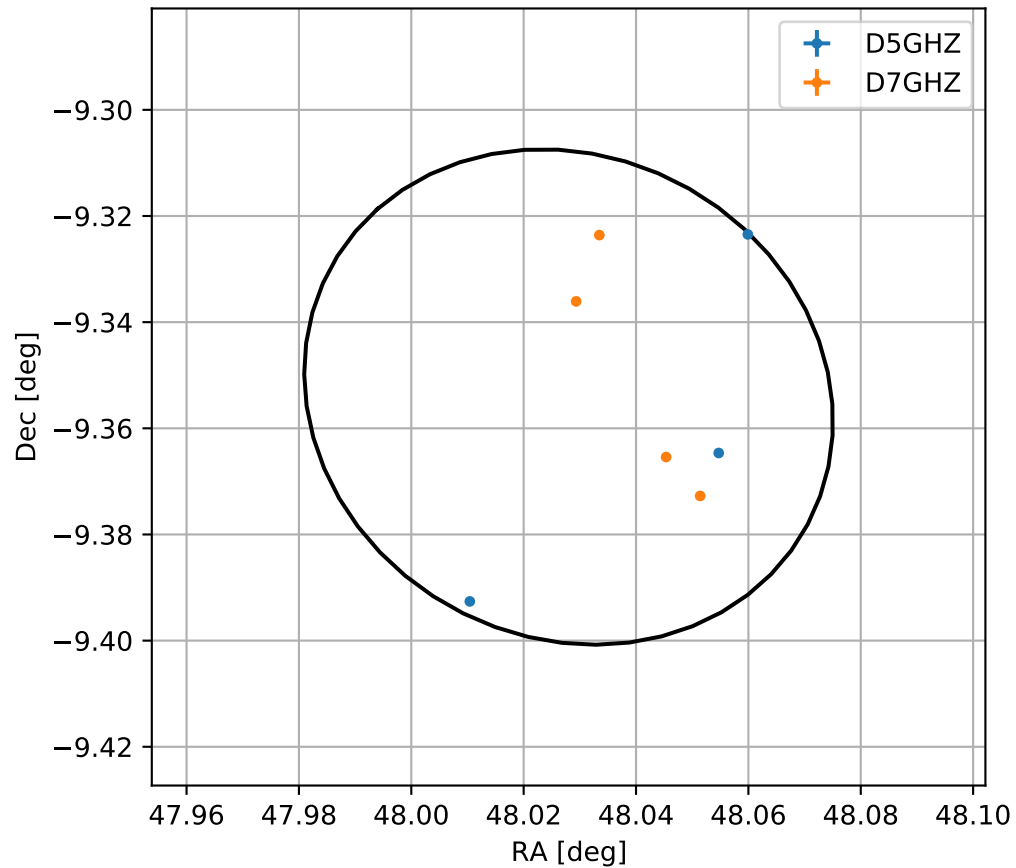
4FGL J0312.1-0921
