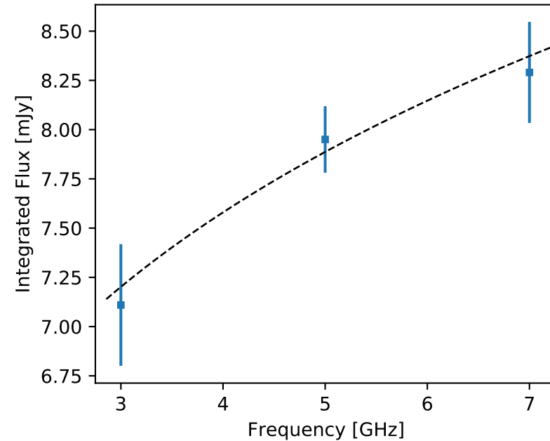
F357 J032848.18-112754.0 (unr)
