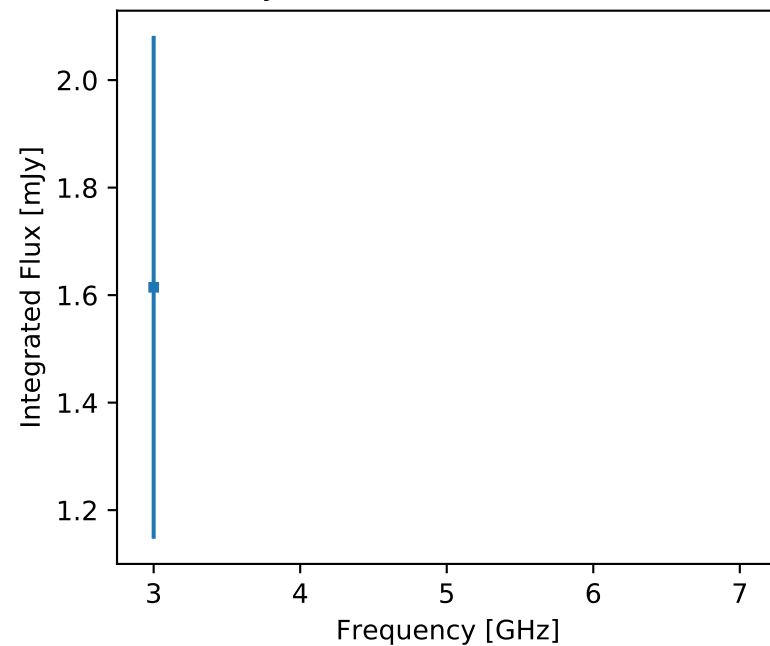
F357 J034210.09+315308.8 (unr)
