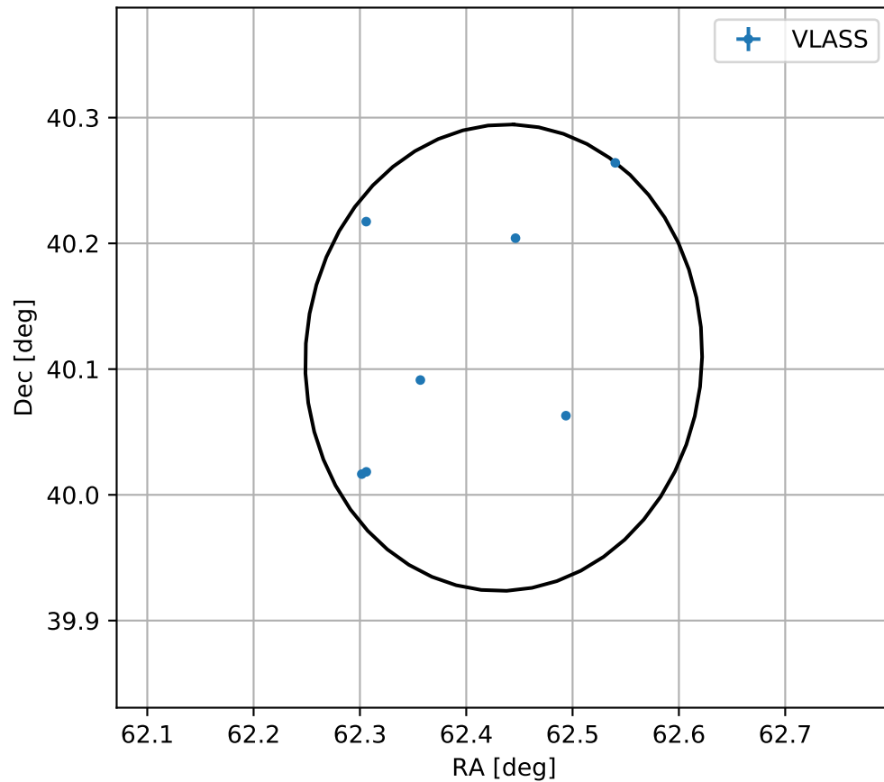
4FGL J0409.7+4006c
