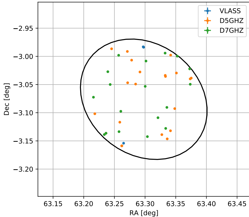
4FGL J0413.1-0304
