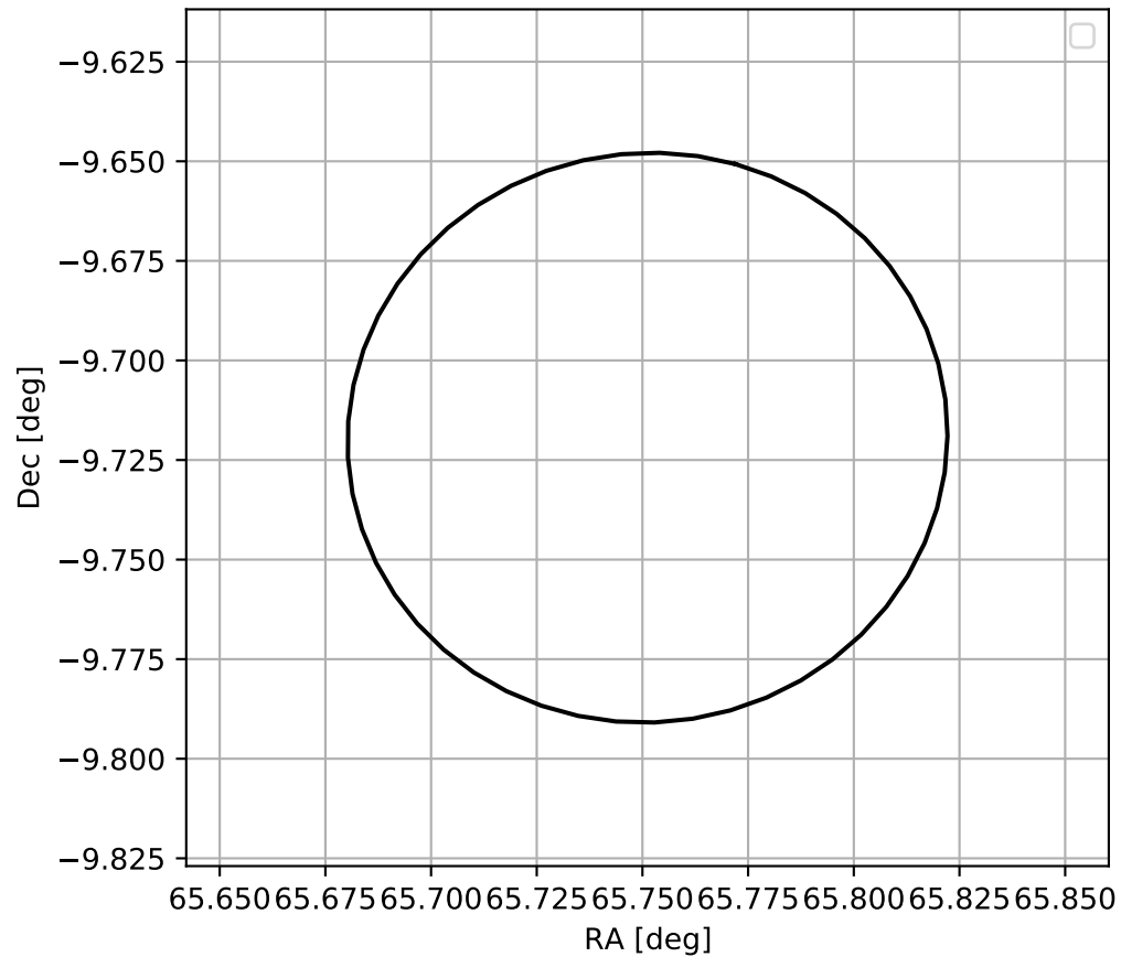
4FGL J0423.0-0943
