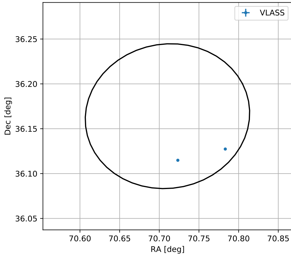
4FGL J0442.8+3609
