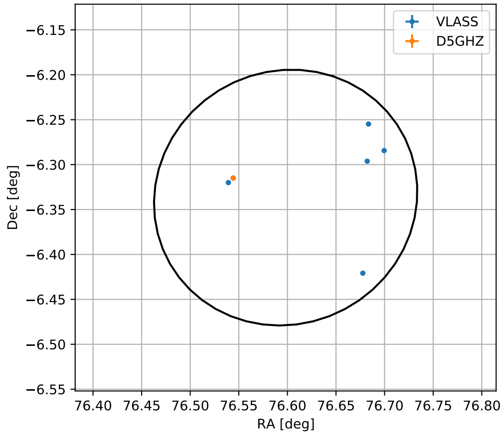
4FGL J0506.3-0620c
