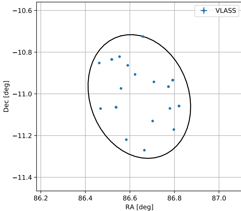
4FGL J0546.5-1100
