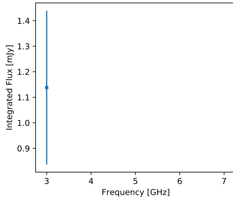
F357 J055328.43+005423.6 (unr)
