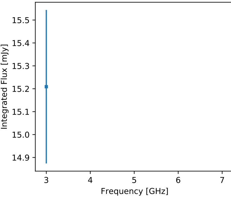
F357 J055340.02+010348.0 (unr)
