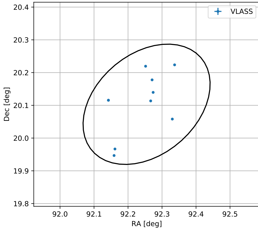
4FGL J0609.0+2006
