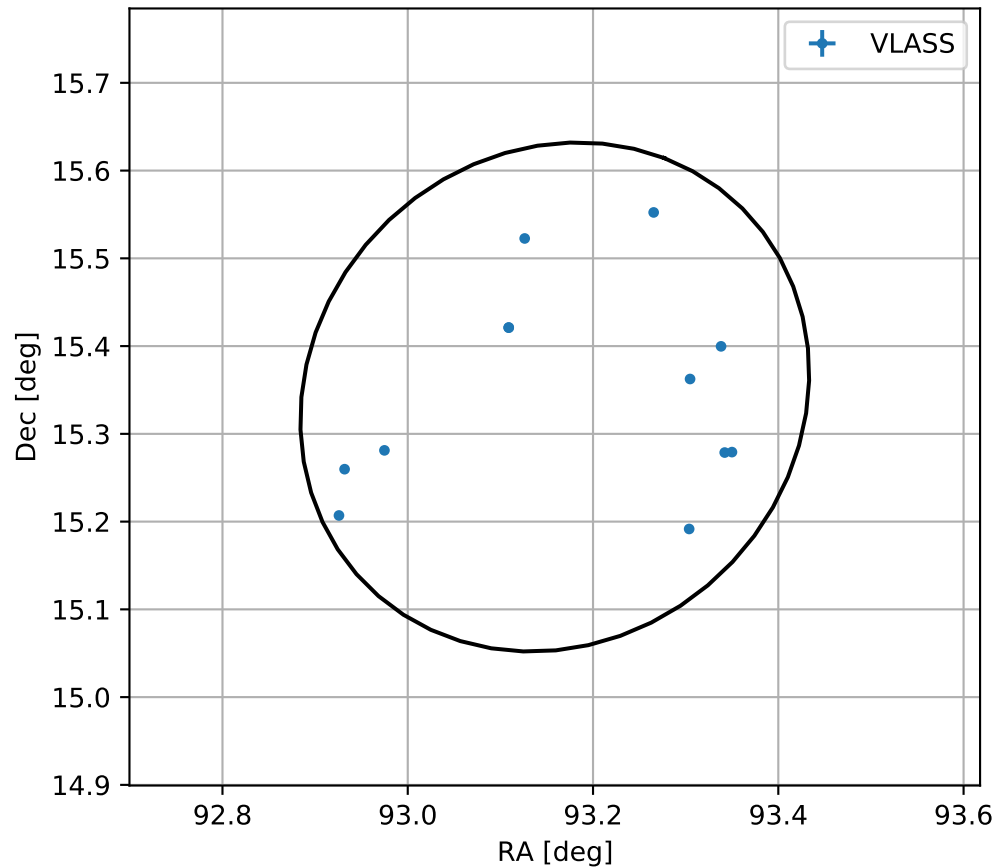
4FGL J0612.6+1520c
