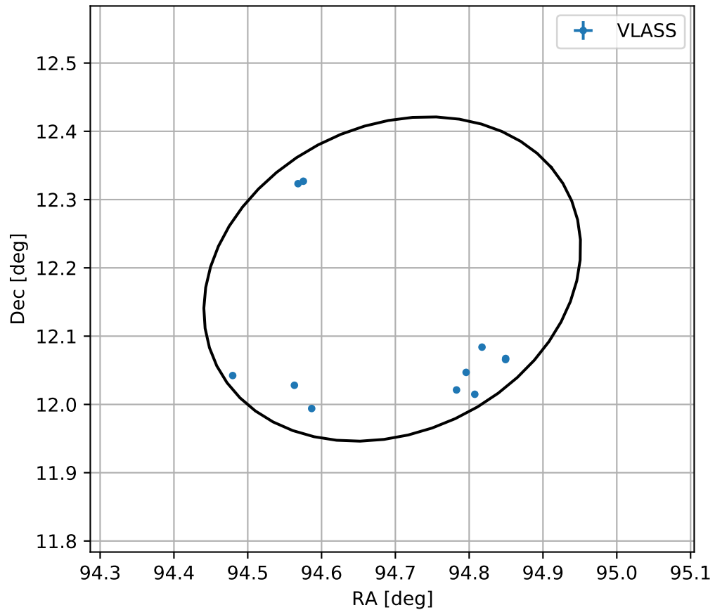
4FGL J0618.7+1211
