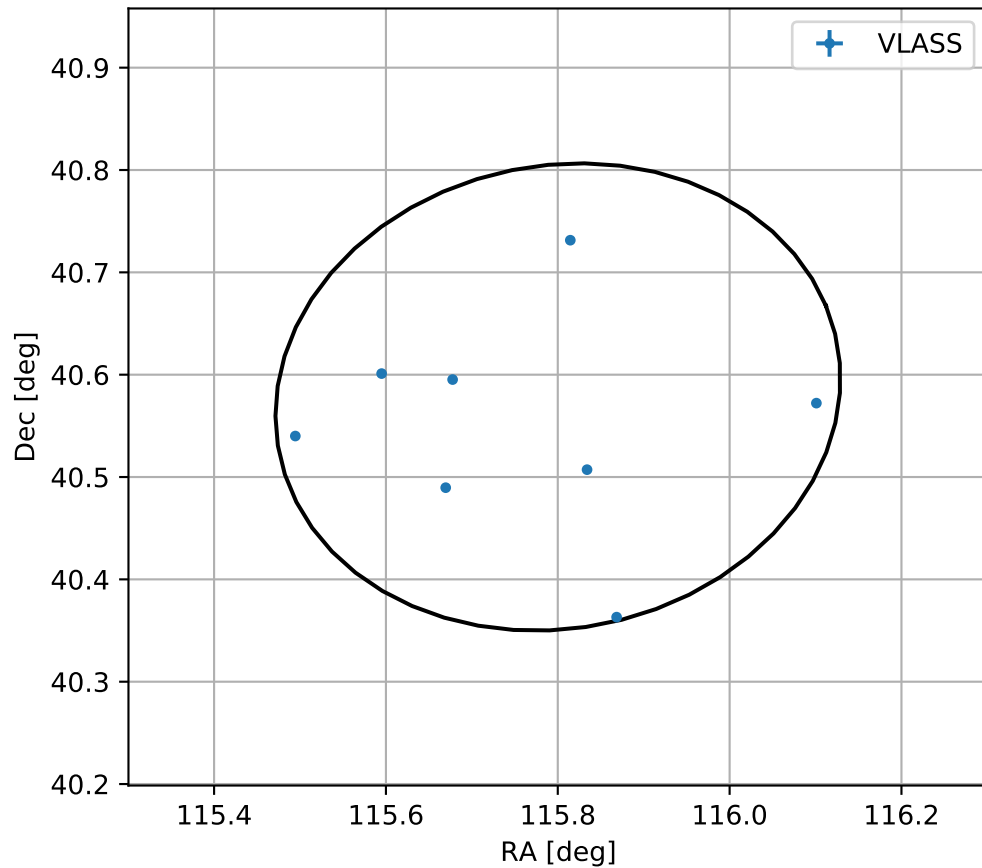
4FGL J0743.2+4034
