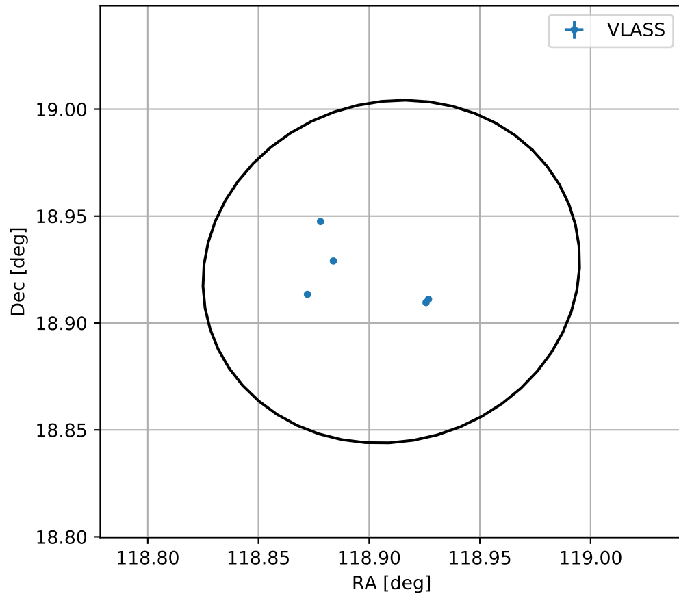
4FGL J0755.6+1855
