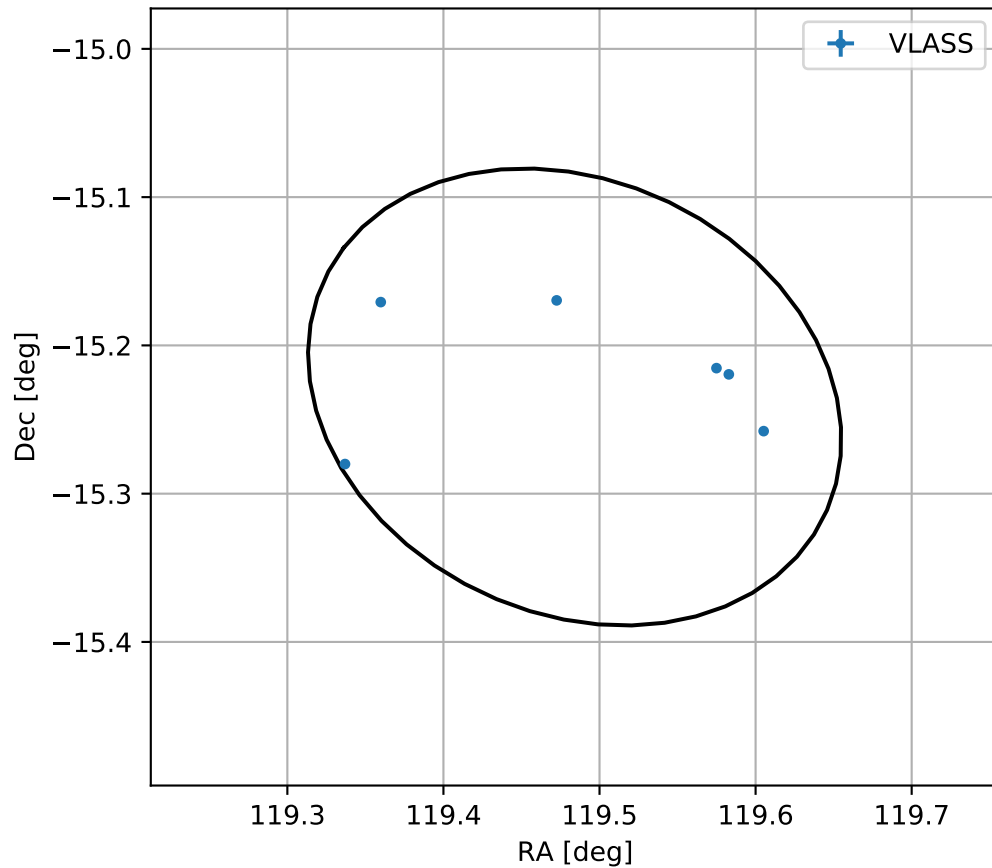
4FGL J0757.9-1514
