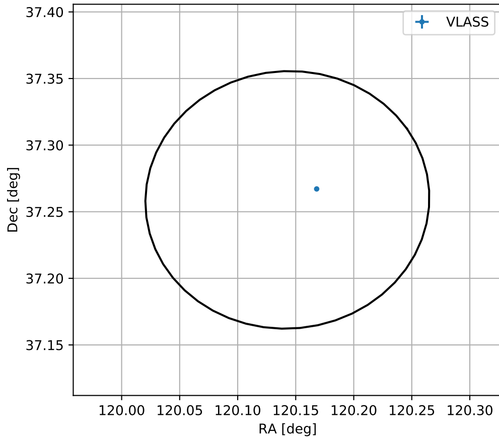
4FGL J0800.5+3715
