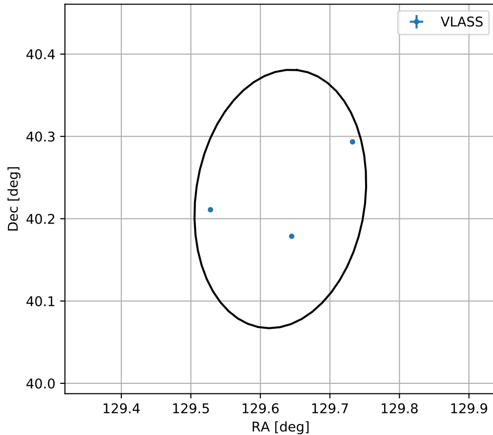
4FGL J0838.5+4013
