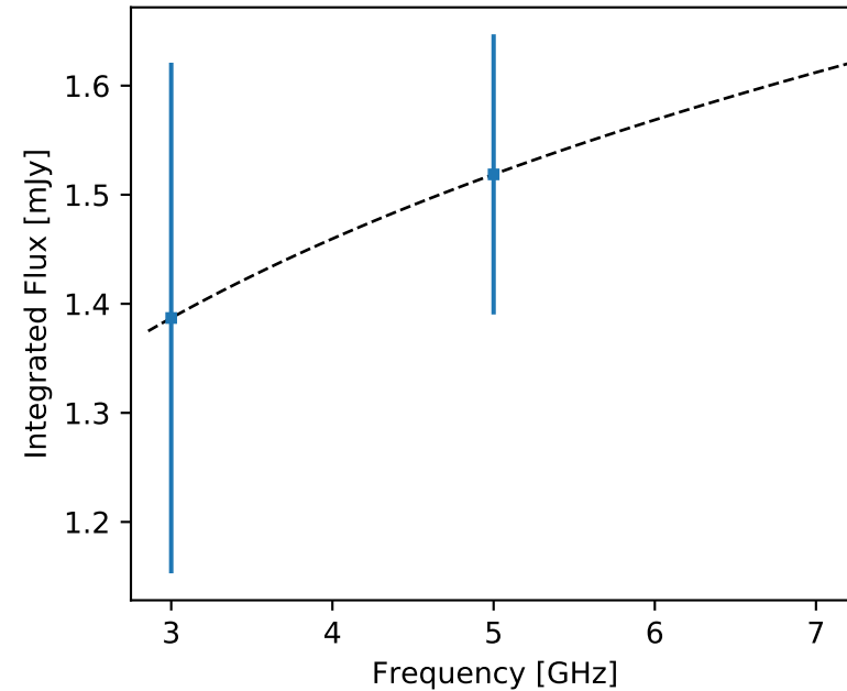
F357 J093531.33+115306.5 (unr)
